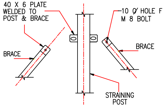
BRACE DETAILS
